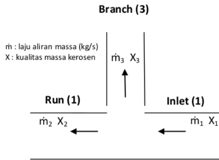
Gambar 1. Model sederhana T-junction [9]
