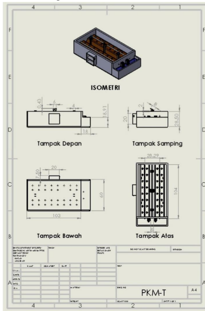
Gambar 2.16 Blueprint Sistem Prototipe Plant Care
