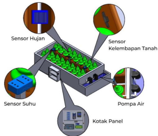
Gambar 2.2 Peralatan Sistem Prototipe Plant Care
