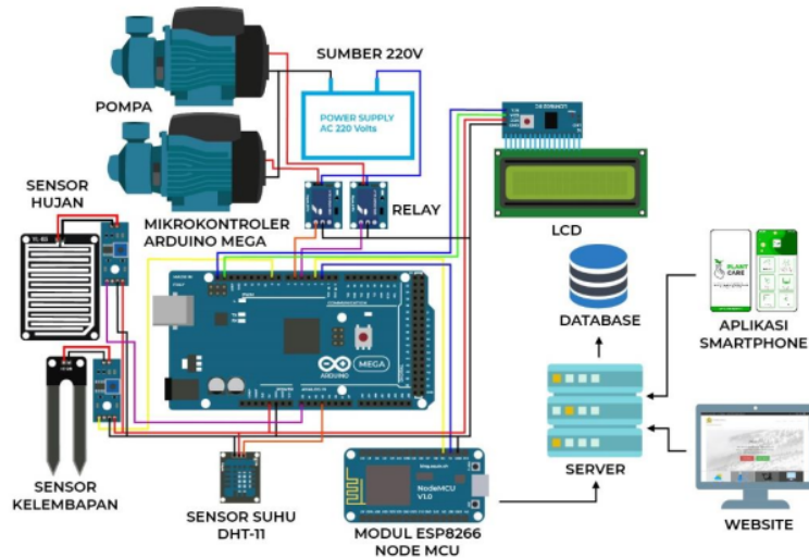
Gambar 3.4 Wiring Sistem Plant Care
