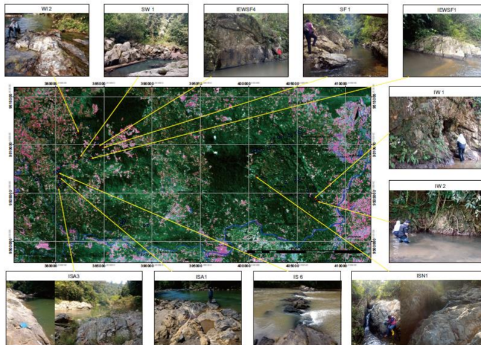
Figure 2. Landsat Image Band 753 and rock sampling locations.
