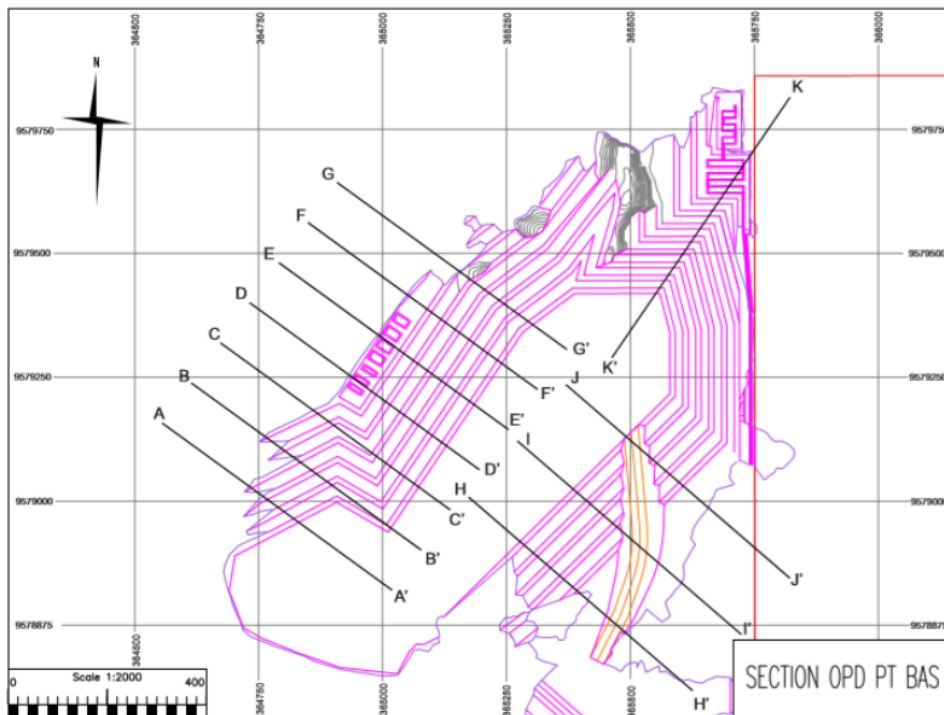
Gambar 4. Section Out Pit Disposal
