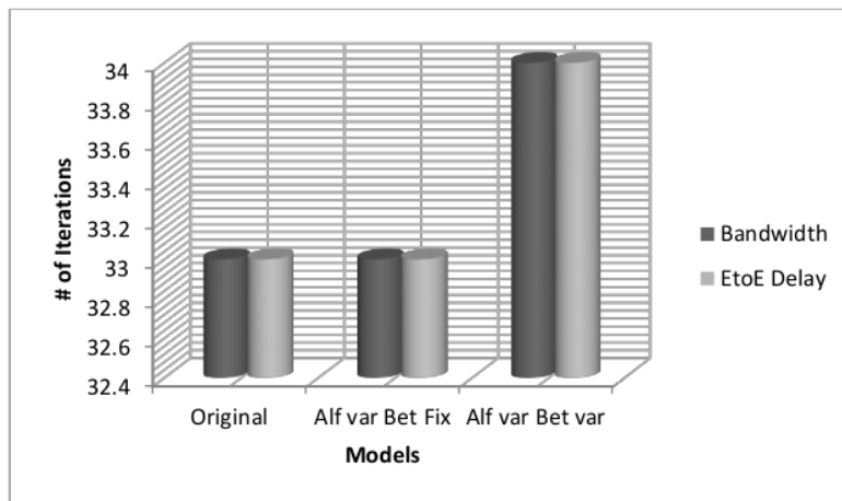
Fig. 2. The comparison of the number of iterations need to complete the computation of three models based on the QoS Attributes
