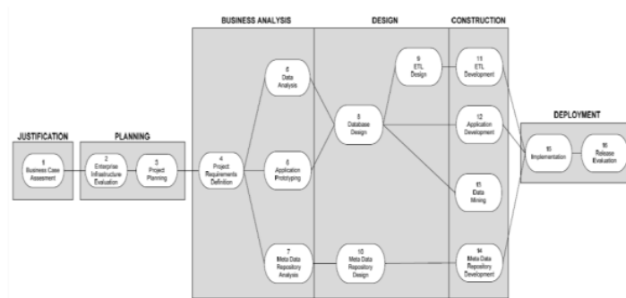
Gambar 1: Business Intelligence Roadmap [5]
