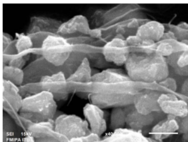
Figure 4. SEM of NCO with 40,000x magnification
