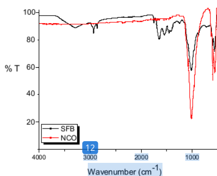
Figure 2. FTIR Spectra of SFB and NCO
