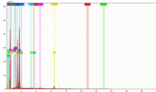
Fig. 14. EDS analysis of Original soil + 6% RHA
