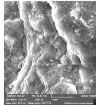
Fig. 9. SEM analysis results of Original soil
