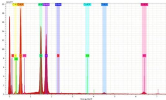
Fig. 13. EDS analysis of Original soil
