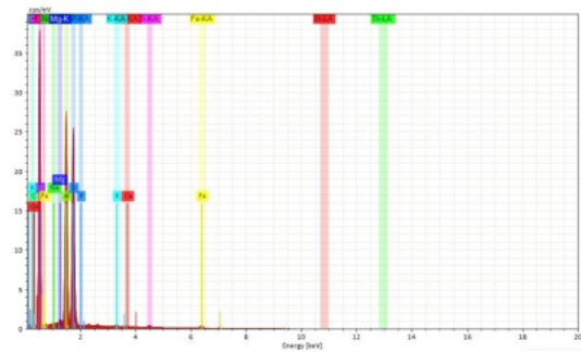
Fig. 15. EDS analysis of Original soil + 9% RHA
