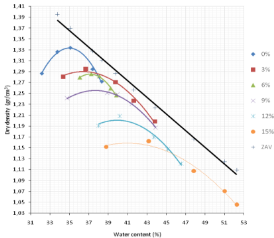
Fig. 5. Graph of the correlation between optimum water content and optimum dry density
