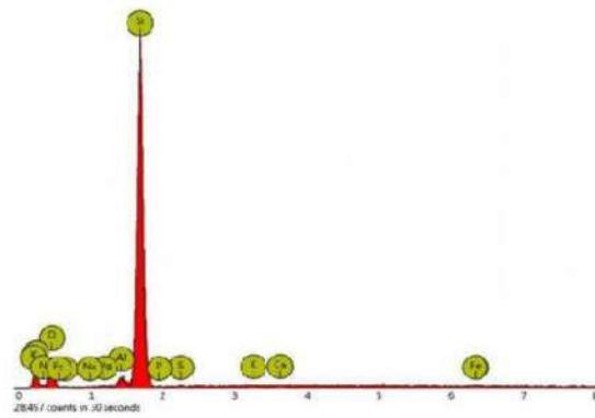
Fig. 5 Result of eds from peat soil in Village iii banyu urip, banyuasin regency
