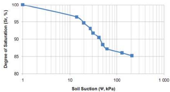
Fig. 11 graph of degree of saturation versus clay soil suction from sample c1
