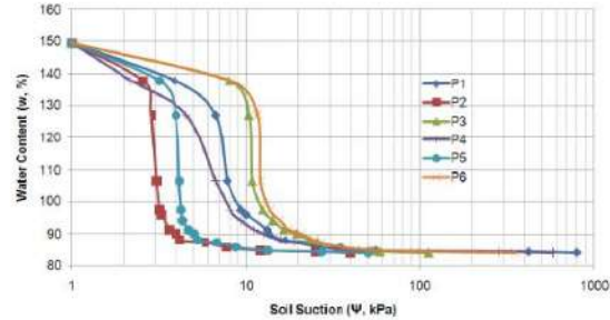
Fig. 13 Soil water characteristic curve (swcc) peat soil suction
