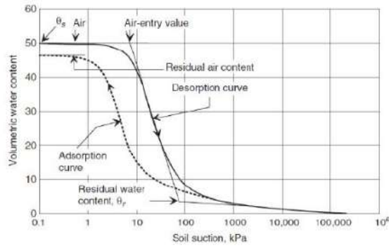
Fig. 1 SWCC characteristic [6]
