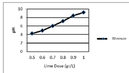
Fig. 1. Results of laboratory tests for the operating time of 30 minutes.
