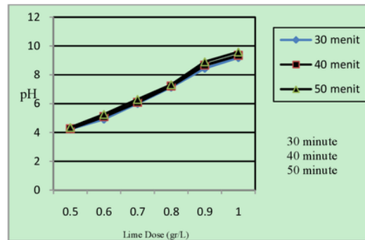
Fig. 4. Comparison chart of lime dose ratio with variation of operating time.
