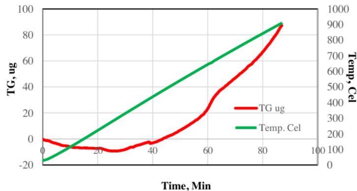
Fig. 1. Thermogram of changes in mass, time and temperature of Al Pure.
