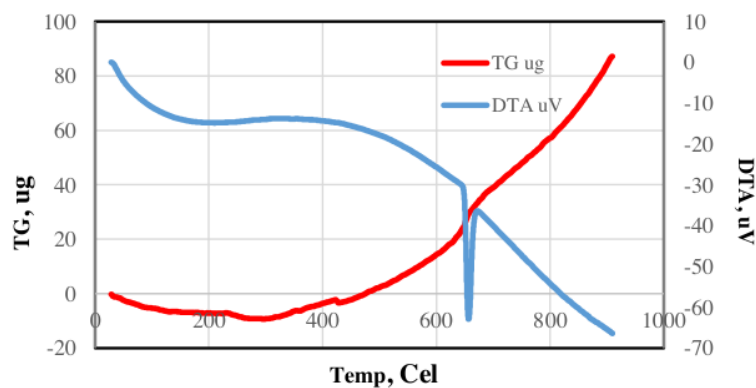
Fig. 2. Melting Point of Pure Aluminum.
