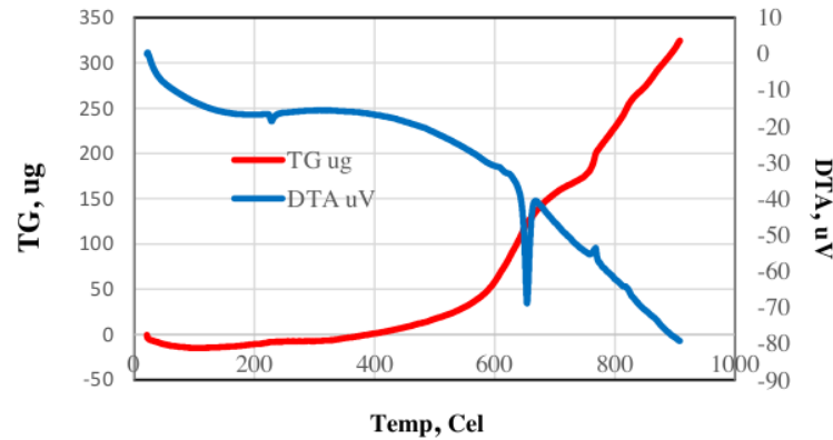
Fig. 11. Melting Point of Alloy 90% Al + 10% Sn.
