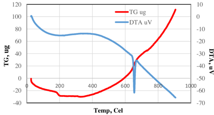
Fig. 5. Melting Point of 98% Al + 2 % Sn.
