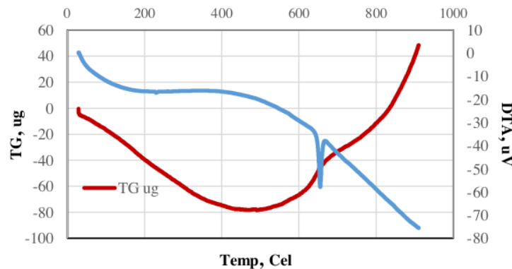
Fig. 8. Melting Point of 94% Al + 6% Sn.
