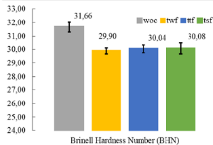
Fig.1 Brinell Hardness Number
