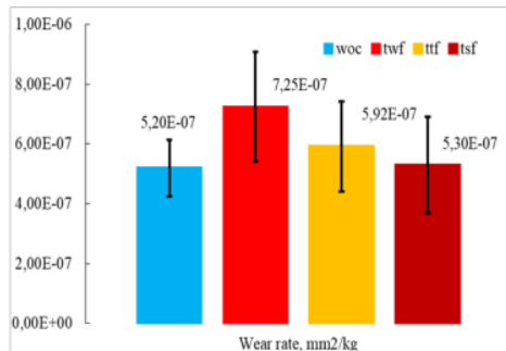
Fig.3 Wear rate
