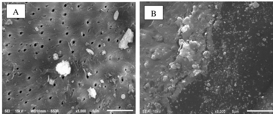
Figure 3. SEM image for (A)chitosan, (B)chitosan-SiO 2 composite.
