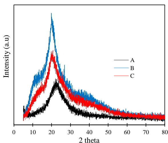
Figure 1. XRD pattern of (A)SiO 2 (B)chitosan (C)chitosan-SiO 2 composite.
