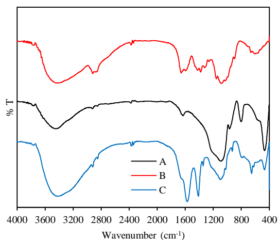
Figure 2. FT-IR spectra of (A)SiO 2 (B)chitosan (C)chitosan-SiO 2 composite.
