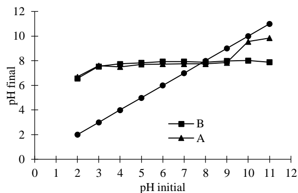
Figure 4. pH_{PZC} (A)chitosan and (B)chitosan-SiO 2 composite.
