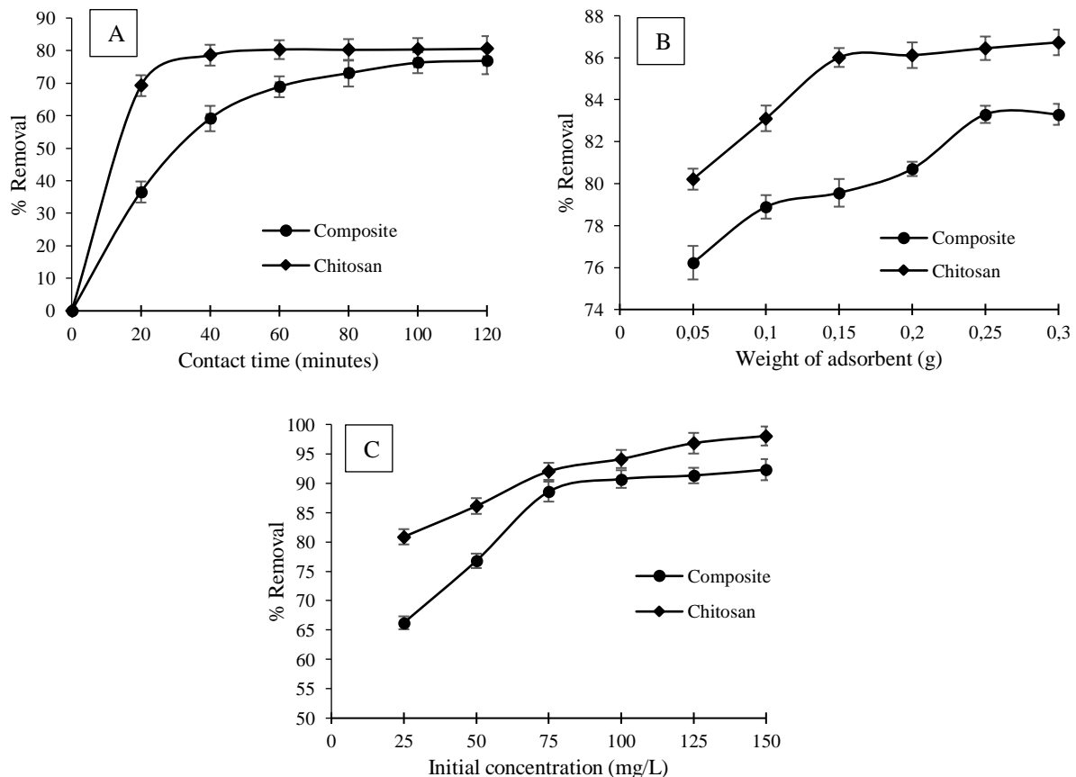
Figure 5. Sorption of methyl red dye onto chitosan and chitosan-SiO 2 composite (A)effect contact time (B)effect weight of adsorbent and (C)effect of initial concentration.
