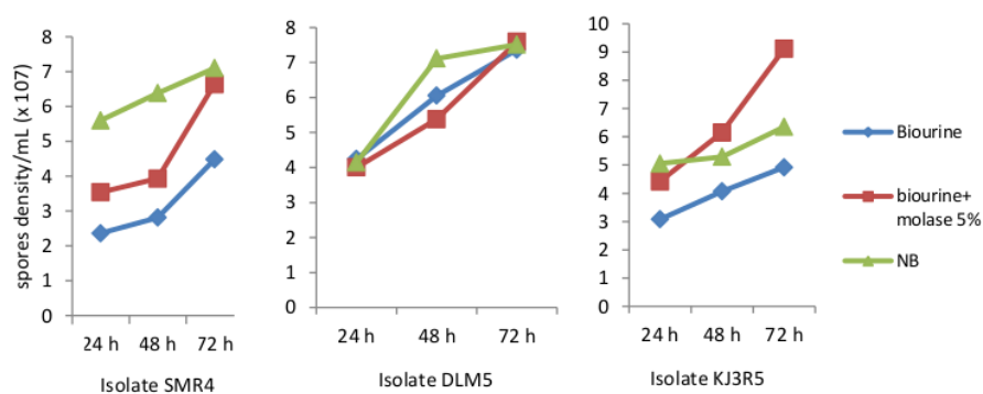
Figure 1. Spores density of Bacillus thuringiensis propagated on various growth media.
