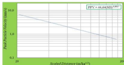
Gambar 3. Korelasi Scaled Distance terhadap PPV
