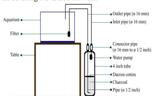
Figure 1. Recirculation system unit
