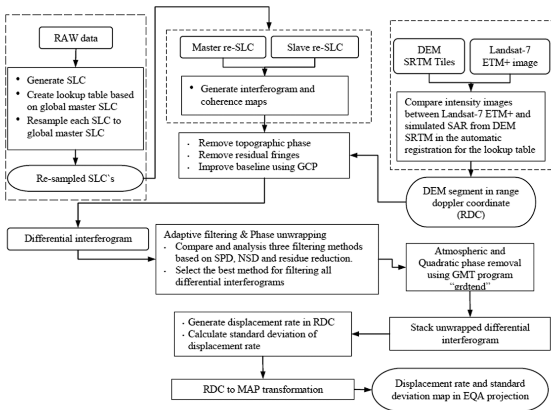
Fig. 1. Processing flowchart for estimating surface deformation.
