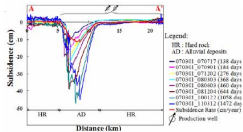
Figure 3: Profiles of time series subsidence across Cimahi city along line A-A' in Figure 2a obtained from stacking 32 differential SAR interferograms and an individual SAR interferogram with the time intervals from 138 to 1472 days with the baseline date of 1 March 2007.
