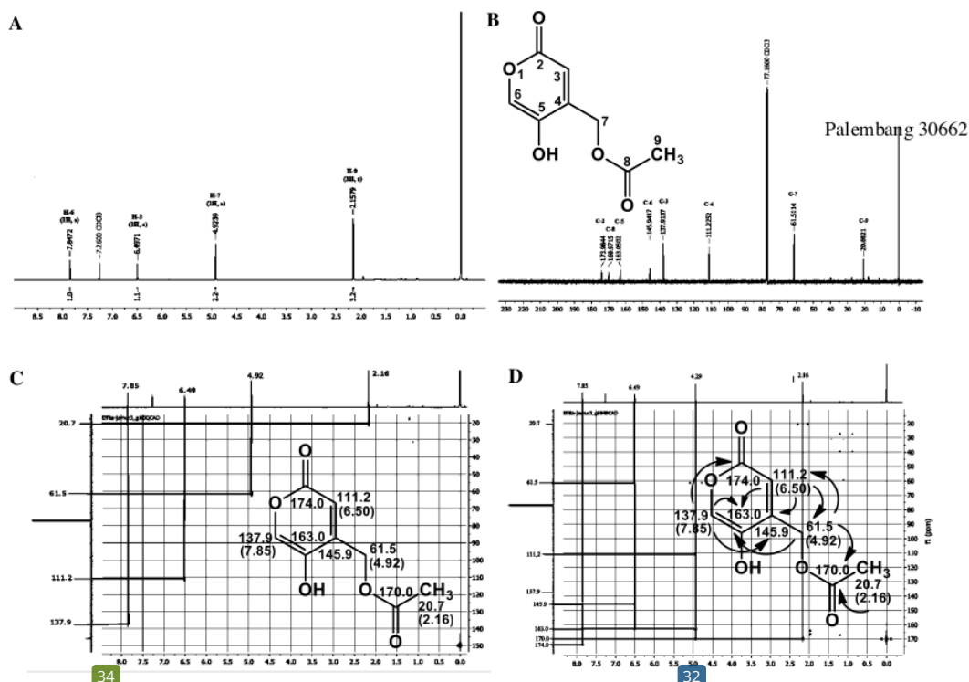
Figure 1. The 1 H-NMR (A), 13 C-NMR (B), HSQC (C), and HMBC (D) spectra of compound 1 ( 1 H-500 MHz, 13 C-125 MHz, in CDCl 3 )
