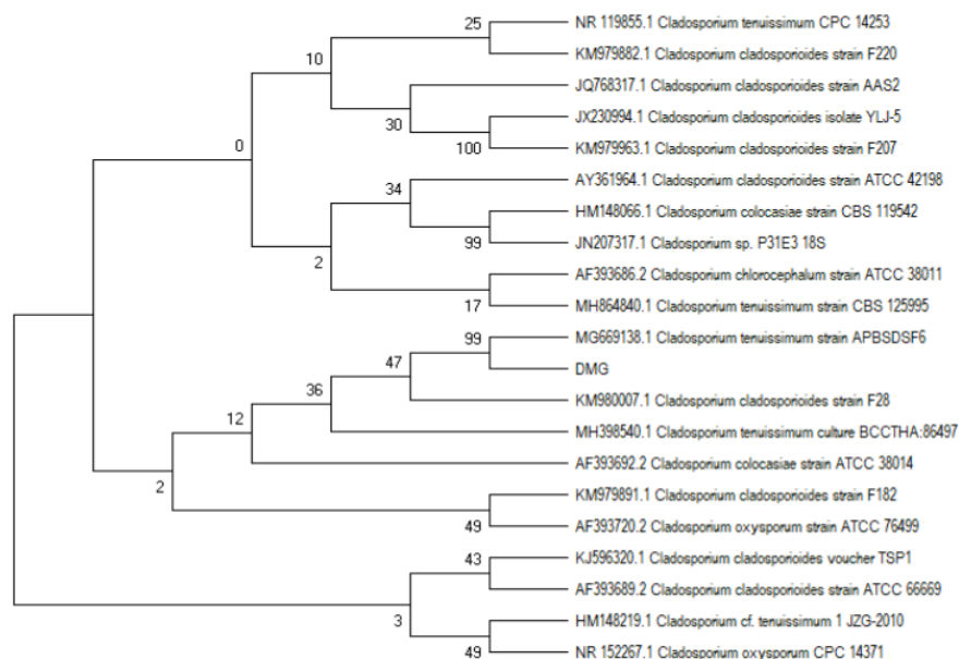
Figure 2. Phylogenetic trees of DMG3
