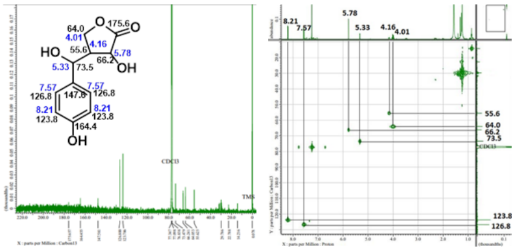
Figure 5. A Spectrum of ^{13}\text{C-NMR} (A) dan HMQC (B) of compound 1
