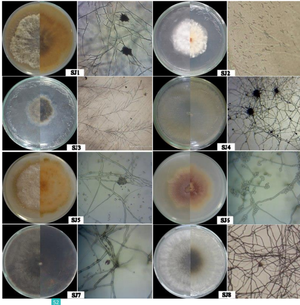
52 Figure 1. Morphological identification of endophytic fungi from the stem bark of S. jambos macroscopically and microscopically
