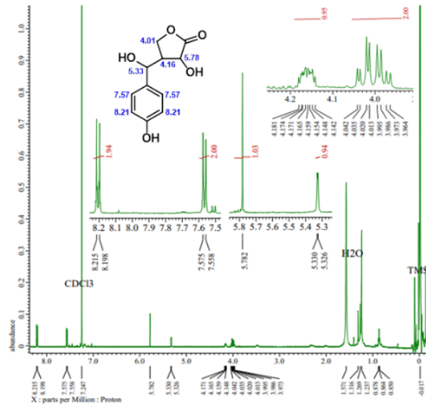
74 Figure 4. The ^1\text{H-NMR} spectrum of compound 1
