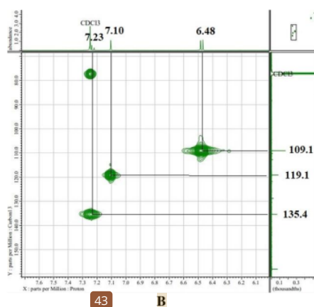
Figure 4. The 13 C-NMR (A) and HMQC (B) spectrum of compound 1 ( 1 H-500 MHz, 13 C-125 MHz in CDCl 3 )
