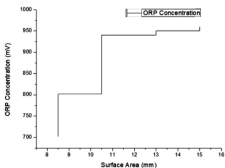
Fig. 3. ORP concentration vs surface area
