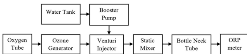
Fig. 2. Experimental setup
