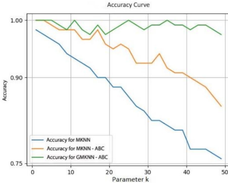
Figure 3. The Accuracy Curve of MKNN, MKNN-ABC and GMKNN-ABC
