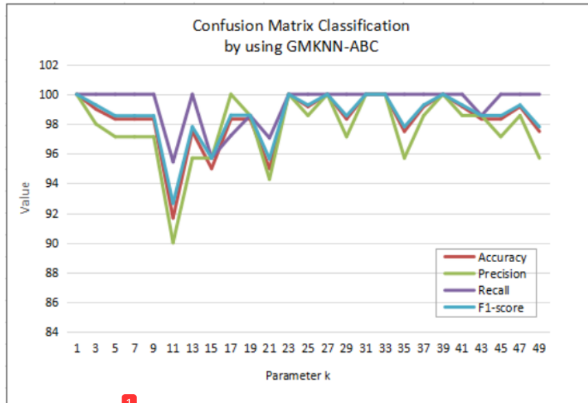
Figure 2. GMKNN-ABC Confusion Matrix Test Results
