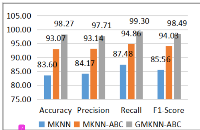
Figure 4. Comparison of Average Confusion Matrix Graphs
