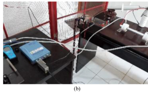
Fig. 3 (a) and (b) Experimental setup DBD reactor
