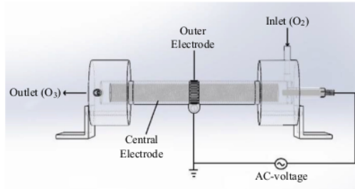
Fig. 1 Design cylinder DBD
