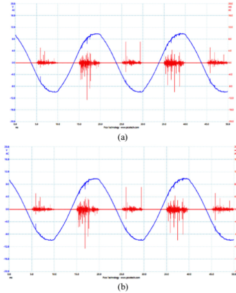
Fig. 4 The effect of voltage and current on ozone concentration (a) Screw 1.5 mm (b) Screw 2 mm
