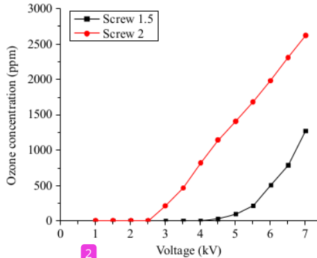
Fig. 5 The effect of voltage on ozone concentration
