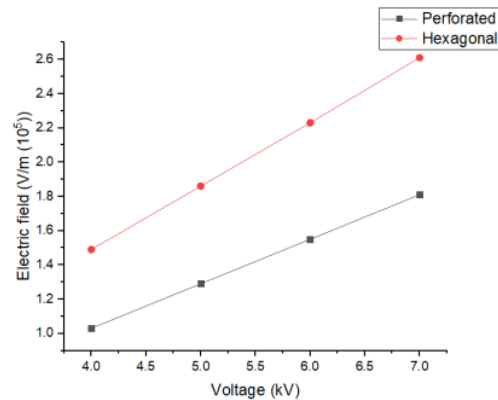
Fig. 9. Effects of electric field on increase voltage
