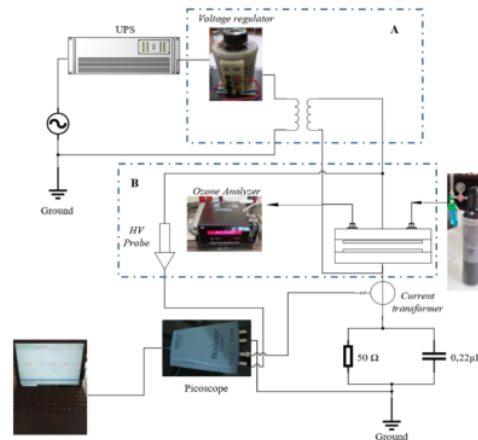
Fig 3. Experimental setup
