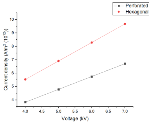
Fig. 10. Effects of current density on increase voltage
