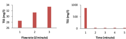
Figure 4. Testing result of TSS level
