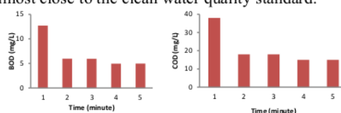
Figure 14. Testing Levels of BOD (mg/l) and COD (mg/l)
