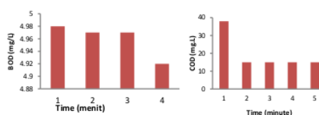
Figure 8. Testing Levels of BOD (mg/l) and COD (mg/l)
