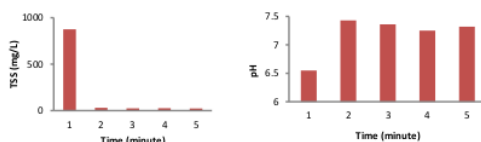
Figure 15. Testing Levels of TSS (mg/l) and pH
