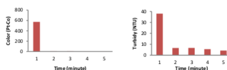
Figure 10. Testing Levels of Color (Pt-Co) and Turbidity (NTU)
