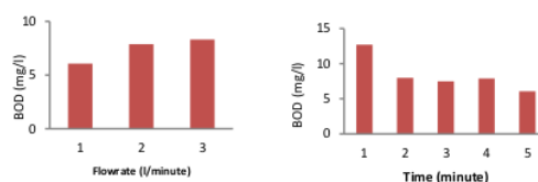
Figure 2. Testing result of BOD level
