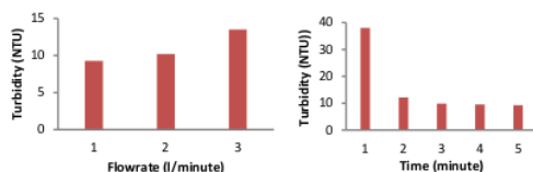
Figure 7. Testing result of turbidity levels
