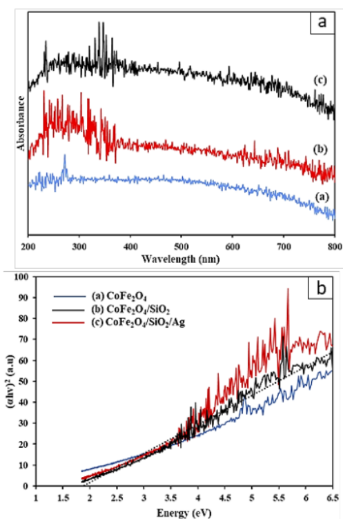
Figure 2 (a) DRS spectra (b) Tauc plot (\alpha hv)^2 versus E_g (eV) of CoFe 2 O 4 , CoFe 2 O 4 /SiO 2 , and CoFe 2 O 4 /SiO 2 /Ag composites
