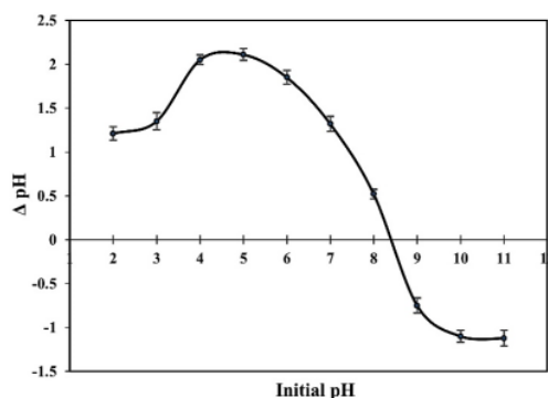
Figure 6. pH_{pzc} of CoFe 2 O 4 /SiO 2 /Ag composite
