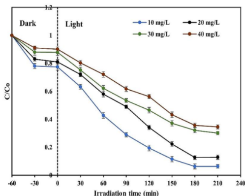
Figure 8. Photocatalytic degradation of Congo red at a different initial dye concentration
