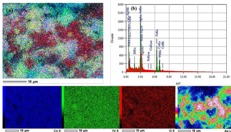
Figure 4. (a) Elemental mapping analysis (b) EDS spectra of CoFe 2 O 4 /SiO 2 /Ag composite
