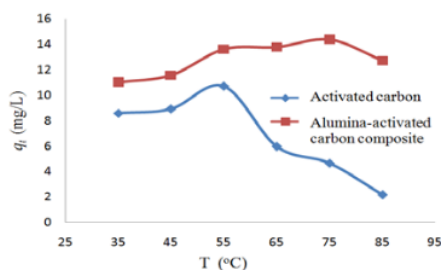
Figure 7. Effect of Temperature
