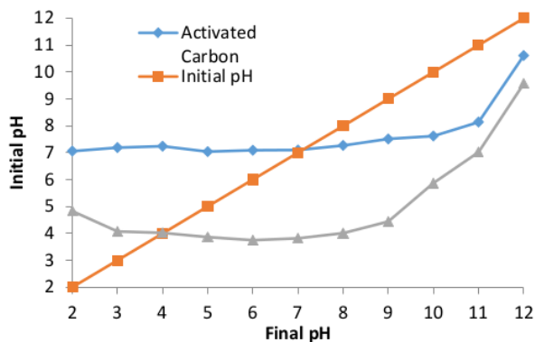
Figure 4. Curve of pH_{PZC}
