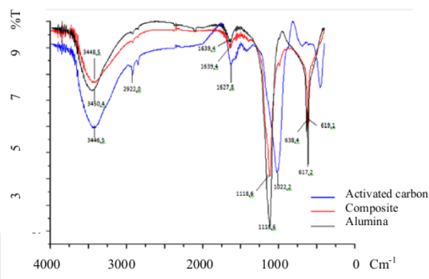
Figure 2. FTIR spectra of Alumina, Alumina-Activated Carbon Composite
