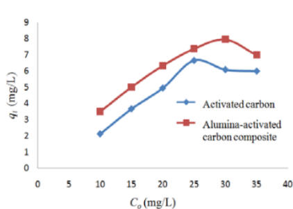
Figure 5. Effect of Concentration
