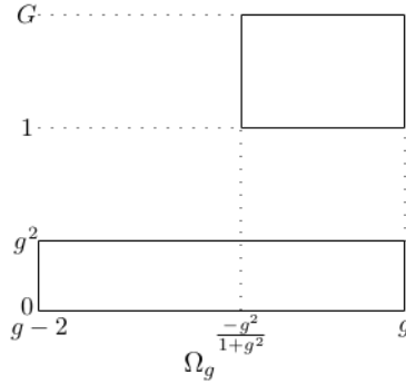
FIGURE 8. The domain \Omega_g .
