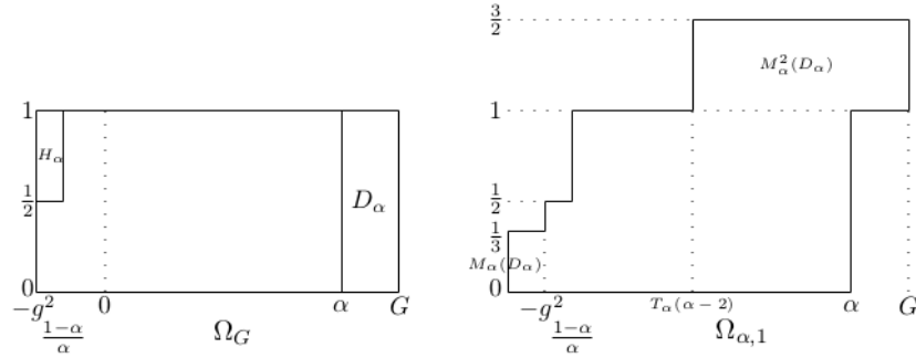
FIGURE 5. The domain \Omega_G and the region \Omega_{\alpha,1} .
