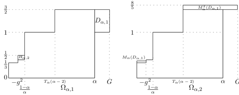
FIGURE 6. The regions \Omega_{\alpha,1} and \Omega_{\alpha,2} .
