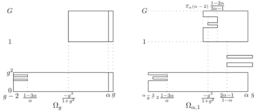
FIGURE 9. The domain \Omega_g and the region \Omega_{\alpha,1} .
