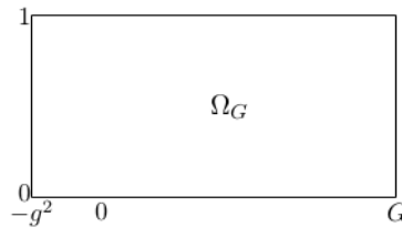
FIGURE 4. The domain \Omega_G .
