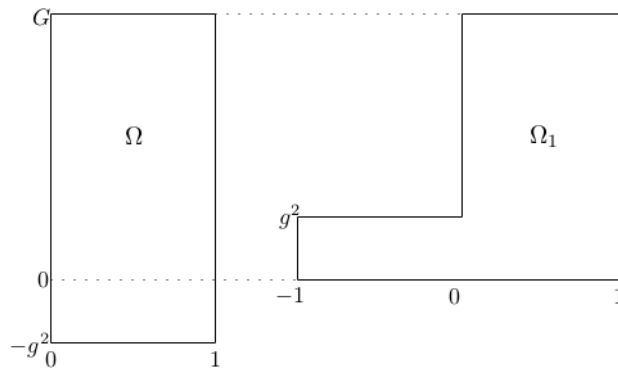
FIGURE 2. The domains \Omega and \Omega_1 .
