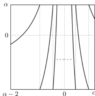
FIGURE 1. The map T_\alpha for \alpha = 0.72 .
