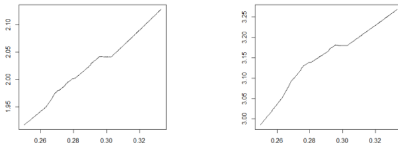
FIGURE 12. Simulations of the entropy as a function of \alpha on the interval [\frac{1}{4}, \frac{1}{3}] . On the left for the odd \alpha -continued fractions, on the right for Nakada's \alpha -continued fractions.
