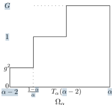
FIGURE 7. The domain \Omega_\alpha for \alpha \in (1, G) .
