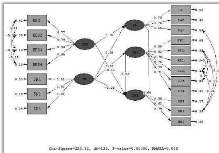
Figure 2. The Estimated Result of Structural Full Model Parameter
