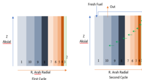
Gambar 2 Skema Modified CANDLE Radial (Tampak Samping)
