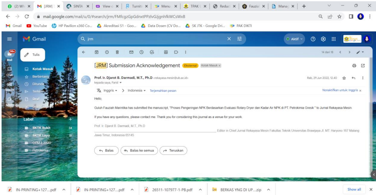
Gambar 3. Submission Acknowledgement
