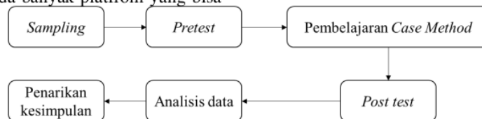
Gambar 1. Prosedur Penelitian
