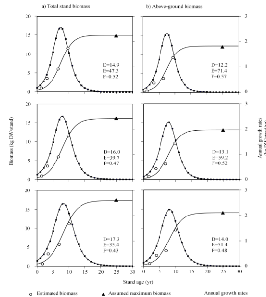
Fig. 3. Growth curves made with both estimated stand biomass, above- and below-ground biomass and total stand biomass in four kind of stand ages of Kandelia candel in Nam Dinh, Vietnam. Maximum stand biomass was assumed in three levels, details referred in Materials & Methods. Values of D, E, and F show the parameters of growth curve equation of Y=D/(1+E \cdot \exp^{-F \cdot t}) , where D is an assumed maximum stand biomass, E=(D-Y_0)/Y_0 where Y_0 is an initial value of stand biomass, t is a stand age, and F is a growth coefficient.
