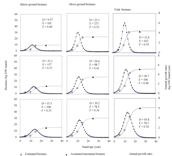
Fig. 2. Growth curves made with both estimated stand biomass, above- and below-ground biomass and total stand biomass in three kinds of stand age in Thanh Hoa, Vietnam. Maximum stand biomass was assumed in three levels, details referred in Materials & Methods. Values of D, E, and F show the parameters of growth curve equation of Y=D/(1+E \cdot \exp^{-F \cdot s}) , where D is an assumed maximum stand biomass, E=(D-Y_0)/Y_0 where Y_0 is an
