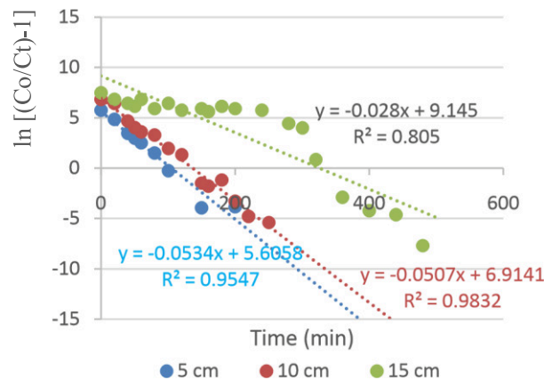
Figure 2. Thomas Kinetic Model
