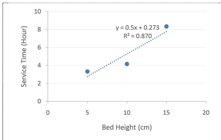
Figure 5. Bed Depth Service Time (BDST) Kinetic Model
