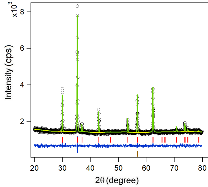
Gambar 5.2. Refinement pola XRD sampel \text{Co}_{0,5}\text{Zn}_{0,5}\text{Fe}_{2-x}\text{La}_x\text{O}_4 ( x = 0,04 )
