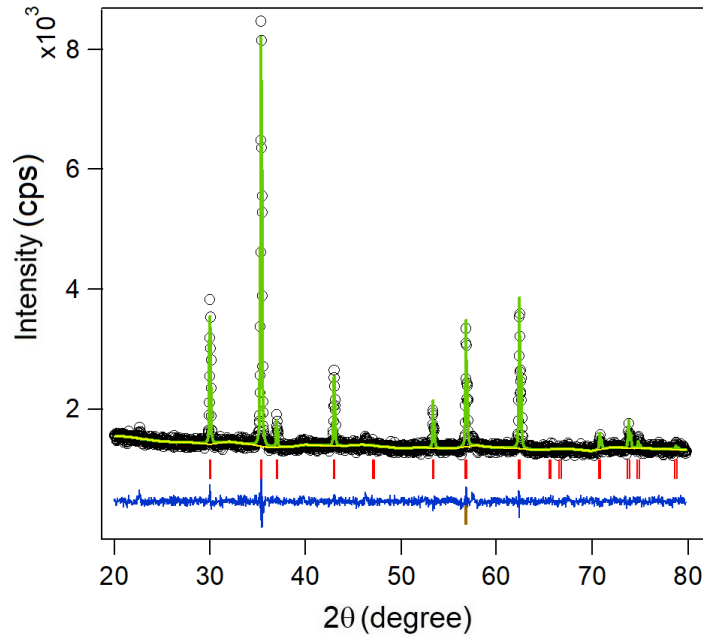
Gambar 5.4. Refinement pola XRD sampel \text{Co}_{0,5}\text{Zn}_{0,5}\text{Fe}_{2-x}\text{La}_x\text{O}_4 ( x = 0,08 )
