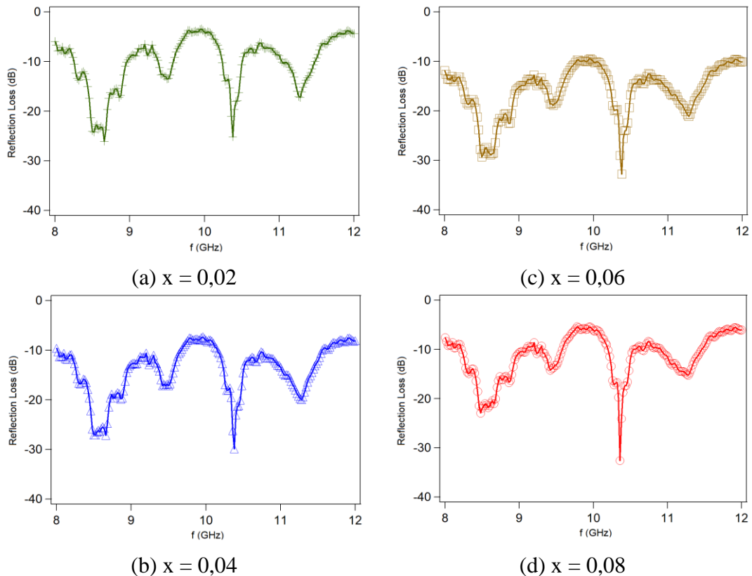
Gambar 5.9. Reflection loss (RL) sampel \text{Co}_{0.5}\text{Zn}_{0.5}\text{Fe}_{2-x}\text{La}_x\text{O}_4 .
