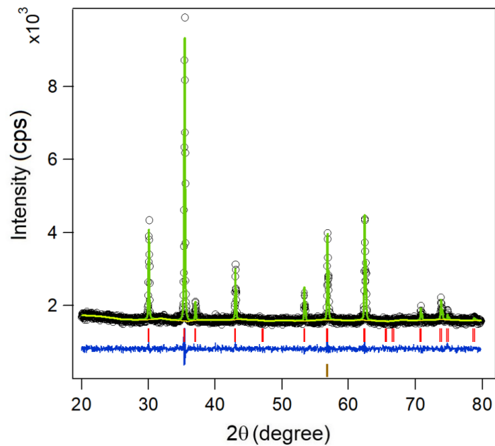
Gambar 5.1. Refinement pola XRD sampel \text{Co}_{0,5}\text{Zn}_{0,5}\text{Fe}_{2-x}\text{La}_x\text{O}_4 ( x = 0,02 )
