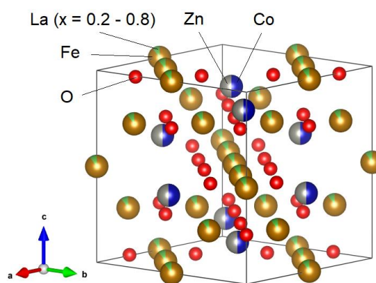
Gambar 5.10. Ilustrasi struktur kristal sampel \text{Co}_{0.5}\text{Zn}_{0.5}\text{Fe}_{2-x}\text{La}_x\text{O}_4
