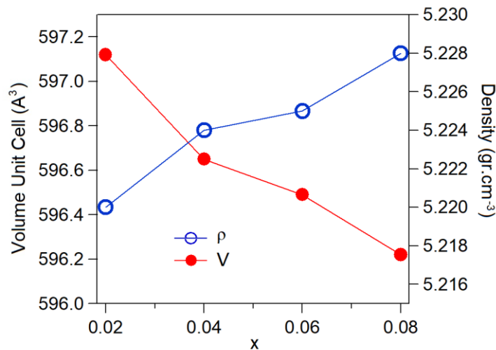
Gambar 5.11. Volume unit sel dan kerapatan atomik sampel \text{Co}_{0.5}\text{Zn}_{0.5}\text{Fe}_{2-x}\text{La}_x\text{O}_4
