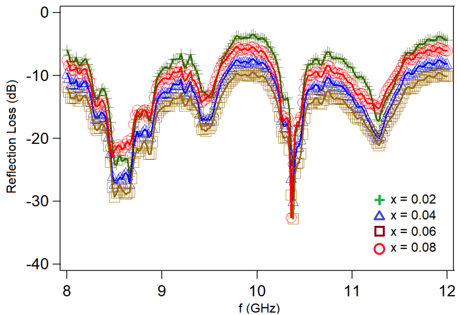
Gambar 5.14. Reflection loss (RL) sampel \text{Co}_{0.5}\text{Zn}_{0.5}\text{Fe}_{2-x}\text{La}_x\text{O}_4
