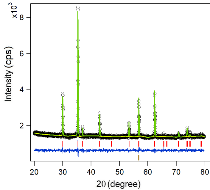
Gambar 5.3. Refinement pola XRD sampel \text{Co}_{0,5}\text{Zn}_{0,5}\text{Fe}_{2-x}\text{La}_x\text{O}_4 ( x = 0,06 )
