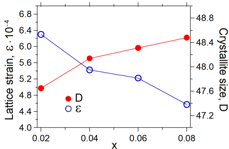
Gambar 5.12. Ukuran kristalit dan strain kisi sampel \text{Co}_{0.5}\text{Zn}_{0.5}\text{Fe}_{2-x}\text{La}_x\text{O}_4
