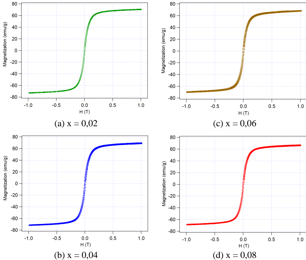
Gambar 5.8. Kurva histerisis sampel \text{Co}_{0.5}\text{Zn}_{0.5}\text{Fe}_{2-x}\text{La}_x\text{O}_4 .
