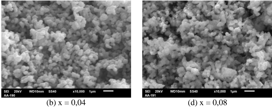
Gambar 5.6. Morfologi permukaan sampel \text{Co}_{0,5}\text{Zn}_{0,5}\text{Fe}_{2-x}\text{La}_x\text{O}_4 .
