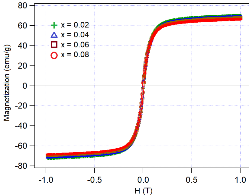
Gambar 5.13. Kurva histerisis sampel \text{Co}_{0.5}\text{Zn}_{0.5}\text{Fe}_{2-x}\text{La}_x\text{O}_4
