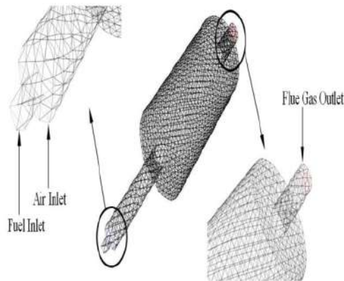
Fig. 2: Mesh Generation of Calculation Domain.
