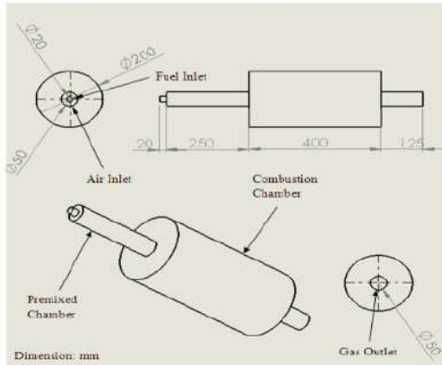
Fig. 1: Solid of Calculation Domain.
