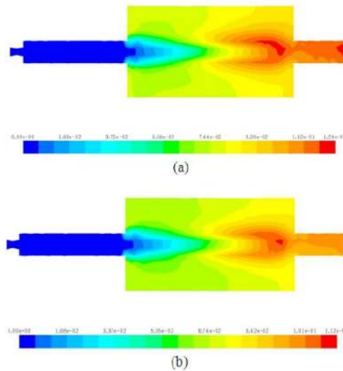
Fig. 5: The 3D of Temperature Distribution on A Axial and A Radial Direction (K).
