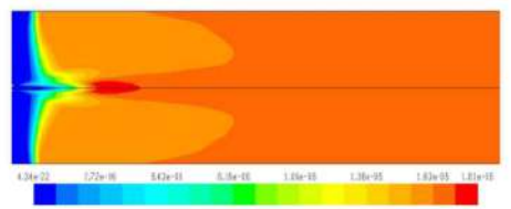
Fig. 22. Nitric oxide distribution in gas burner on excess air of 30%
