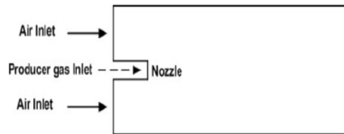
Fig.1. The scheme of gas burner
