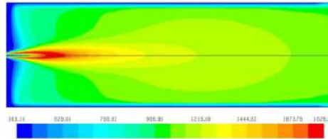
Fig.5. Temperature distribution on excess air of 0%
