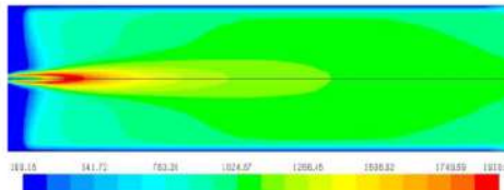
Fig.8. Temperature distribution on excess air of 50%
