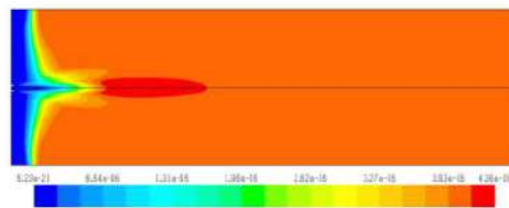
Fig. 21. Nitric oxide distribution in gas burner on excess air of 10%
