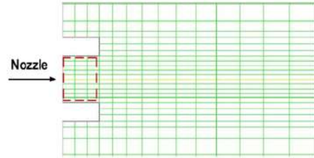
Fig.3. Mesh of the nozzle
