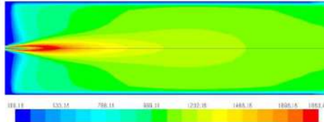
Fig.6. Temperature distribution on excess air of 10%
