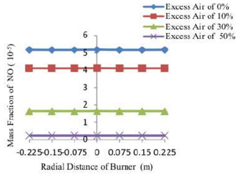
Fig. 19. Nitric Oxide distribution on middle of gas burner at radial distance with difference excess air.
