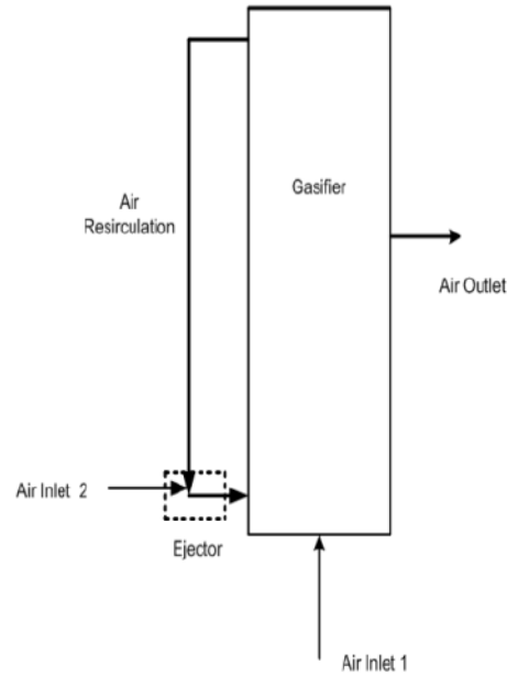
FIGURE 1. Recirculation Model.
