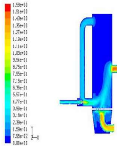
FIGURE 6. Velocity Contour in Reactor with Recirculation Pipe and Ejectors.
