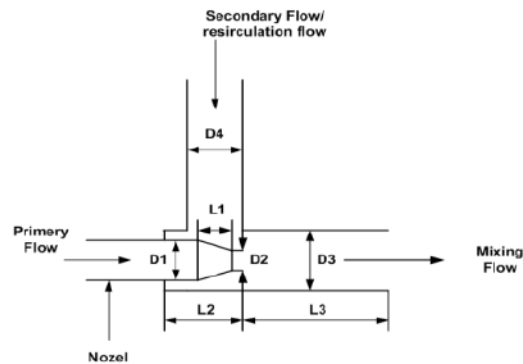
FIGURE 2. Ejector Model.
