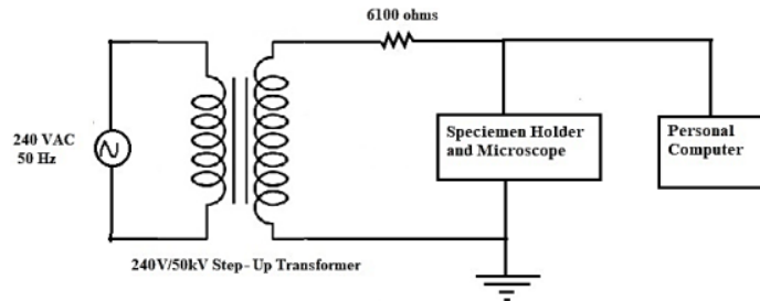
Figure 2. Circuit diagram of experiment set-up
