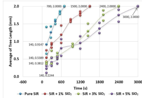
Figure 7. Comparison of average of tree length against time
