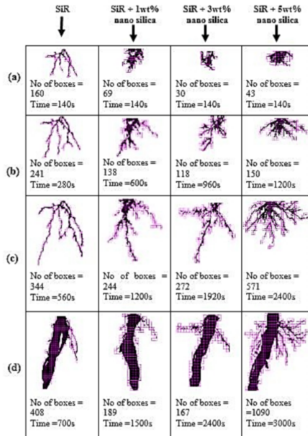
Figure 3. Images of electrical tree propagation with box-counting method in silicone rubber without and with nanocomposites; (a) inception stage, (b) propagation stage 1, (c) propagation stage 2, (d) breakdown stage
