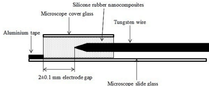
Figure 1. Leaf-like specimen configuration
