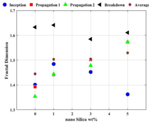
Figure 4. Graph of fractal dimension for silicone rubber with different wt% SiO 2
