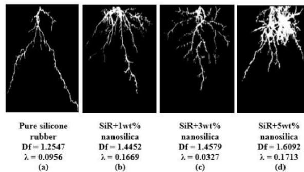
Figure 6. Sample images of different type of electrical treeing; (a) branch type, (b) bush-branch type, (c) bush-branch type, (d) bush-branch type
