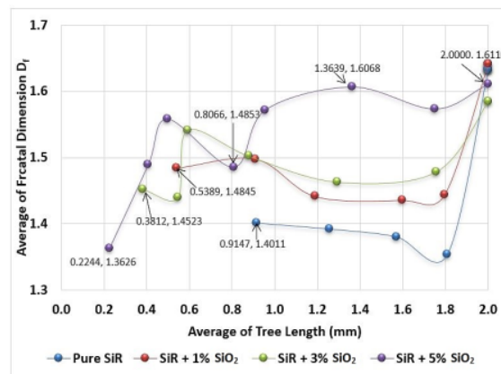
Figure 8. Comparison of average of fractal dimension against tree length
