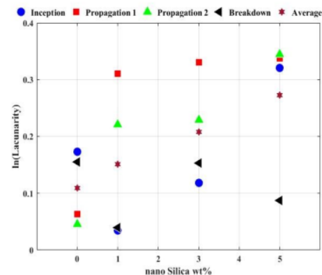
Figure 5. Graph of lacunarity for pure SiR and SiR with different SiO 2 wt% nanofiller
