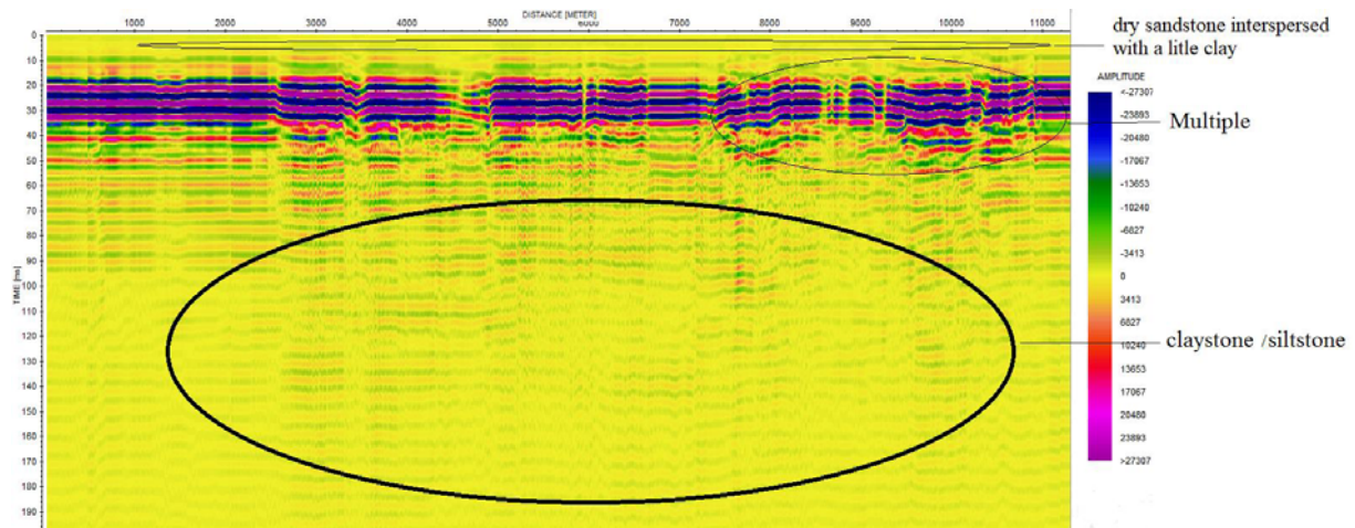
Figure 4. Results of GPR data processing
