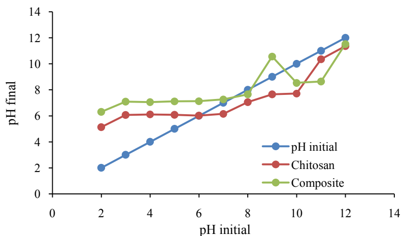
Figure 3. pH pzc of chitosan and chitosan/alumina composite
