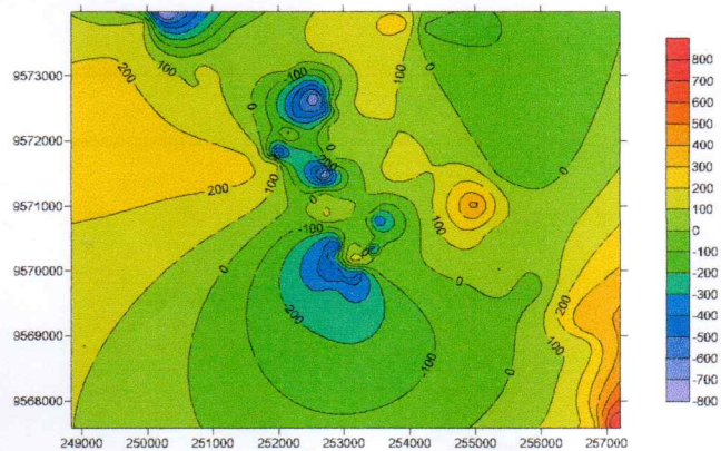
Figure 2. Total magnetic anomaly map of Penantian area.
