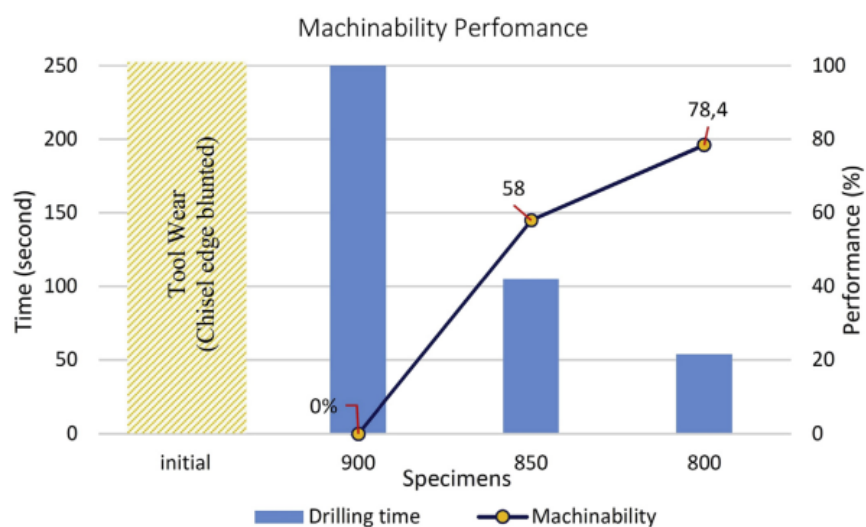
Fig. 6. Machinability performance about drilling process time.
