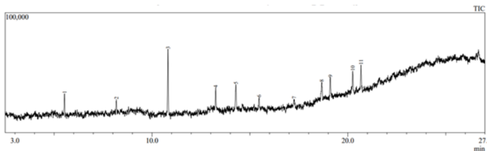
FIGURE 2. GC-MS chromatogram of VCO
