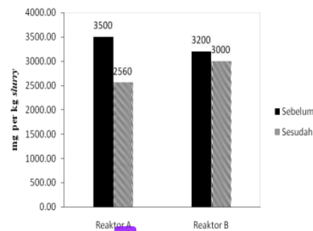
Gambar 4. Nilai Chemical Oxygen Demand (COD).
