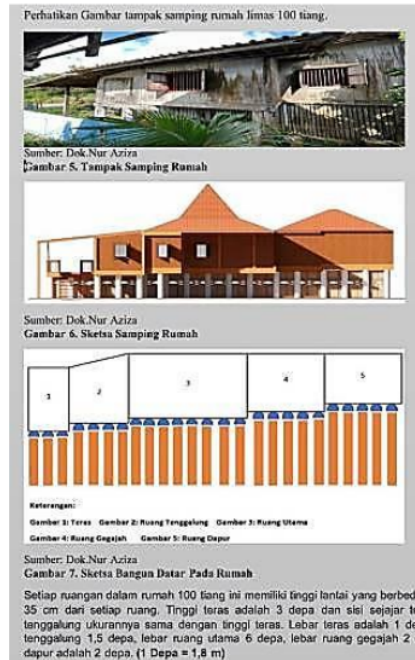
Figure 7. Activity 3 problem 1
