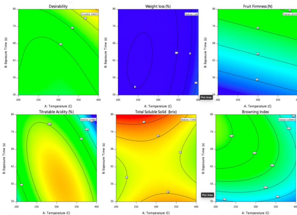
Figure 2 Response surfaces (2D) at 6 cm distance of emitter infrared for the optimization points of exposure time, and temperature on response variables.
