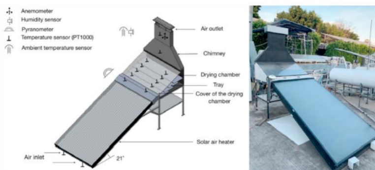
Figure 5. Mixed mode type of solar dryer
