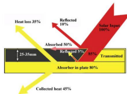
Figure 4. Flat plate collector
