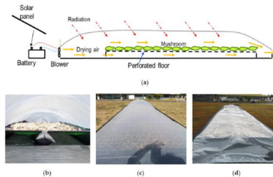
Figure 7. Inflated solar dryers for oyster mushroom drying
