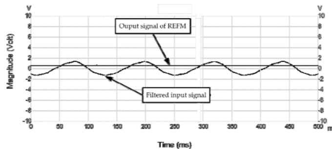
Figure 11. Typical output signal from developing REFM
