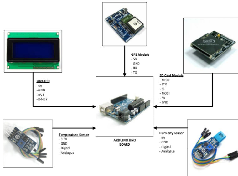
Figure 1. Arduino Uno board and all related sensors and modules
